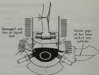
FIGURE 10-45. Results of a hydraulic lock.
